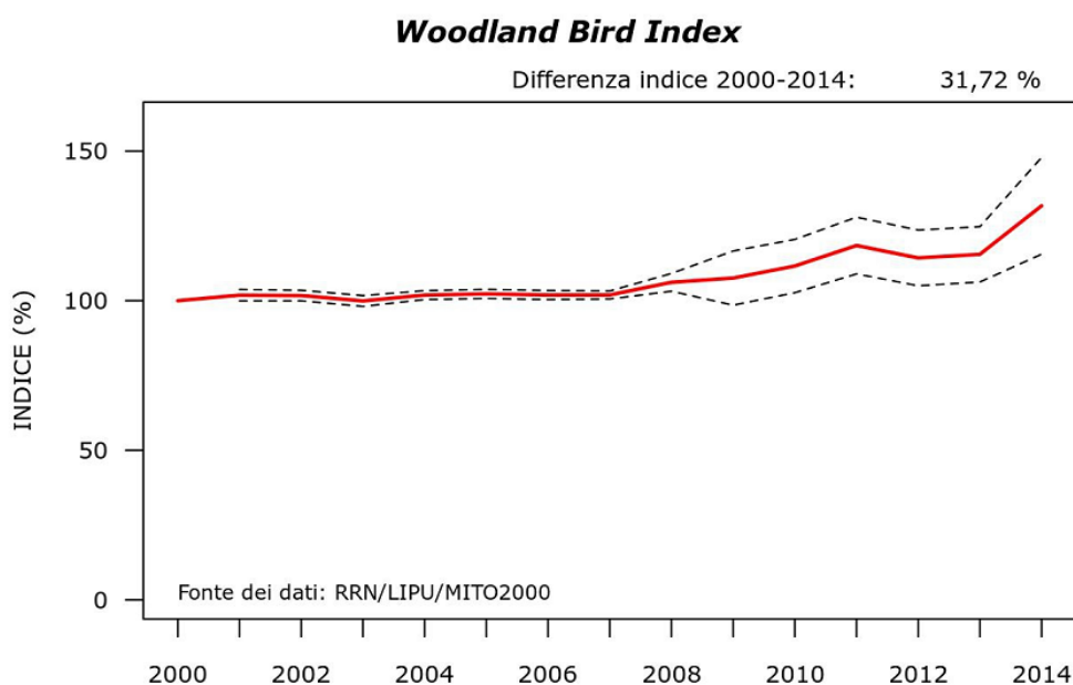
Figura 22. Woodland Bird Index.
